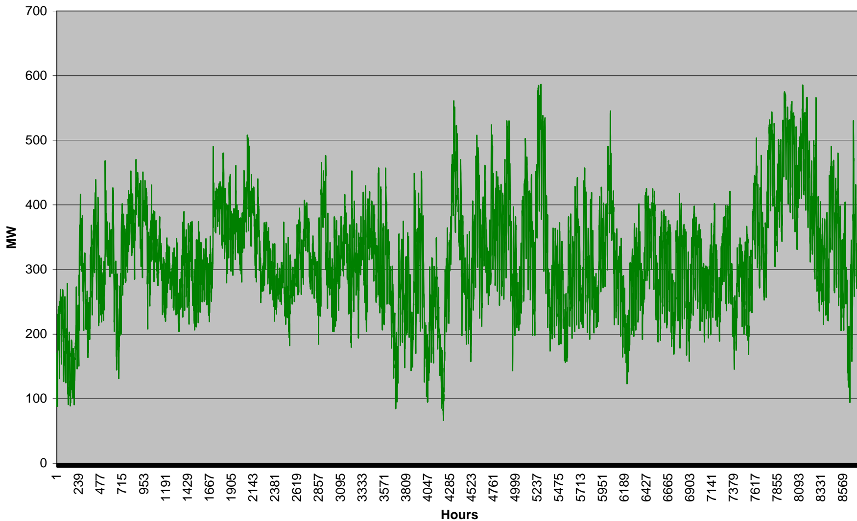
Salem-NMA Alternative: Salem-Spring Green 345 kV Line Flow
