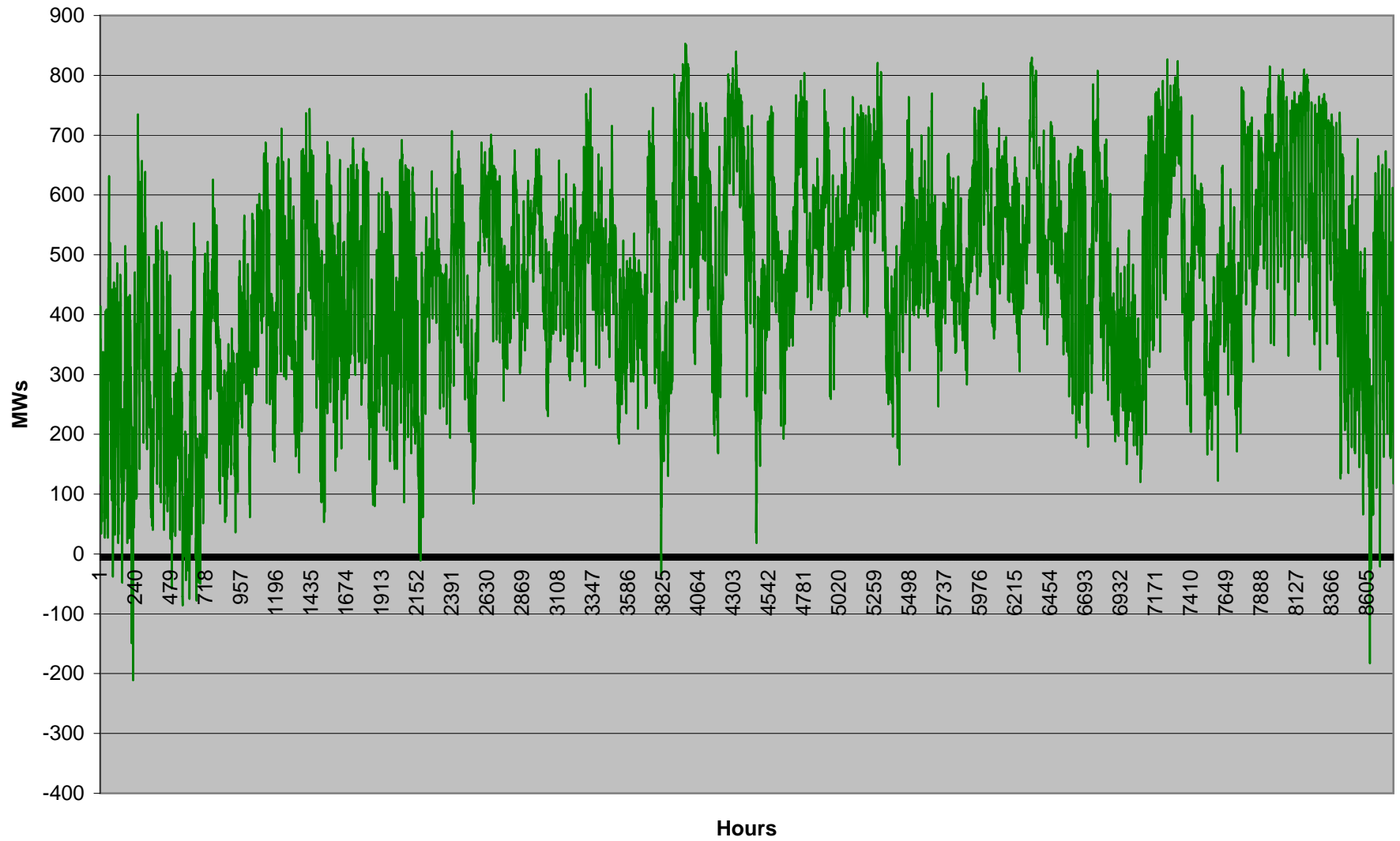
Base Case Alternative: Eau Claire-Arpin 345 Line Flow
