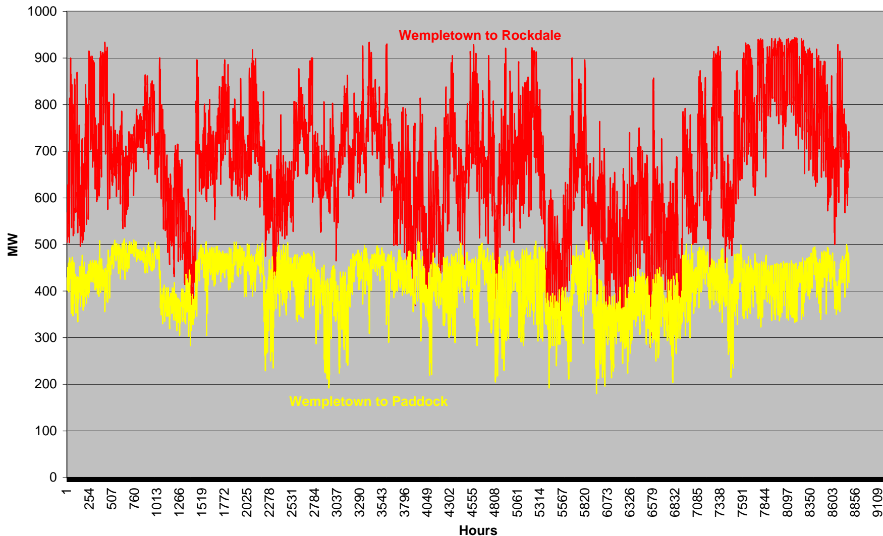
Base Case Alternative: Wempletown-Rockdale & Wempletown-Paddock 345 kV Line Flows
