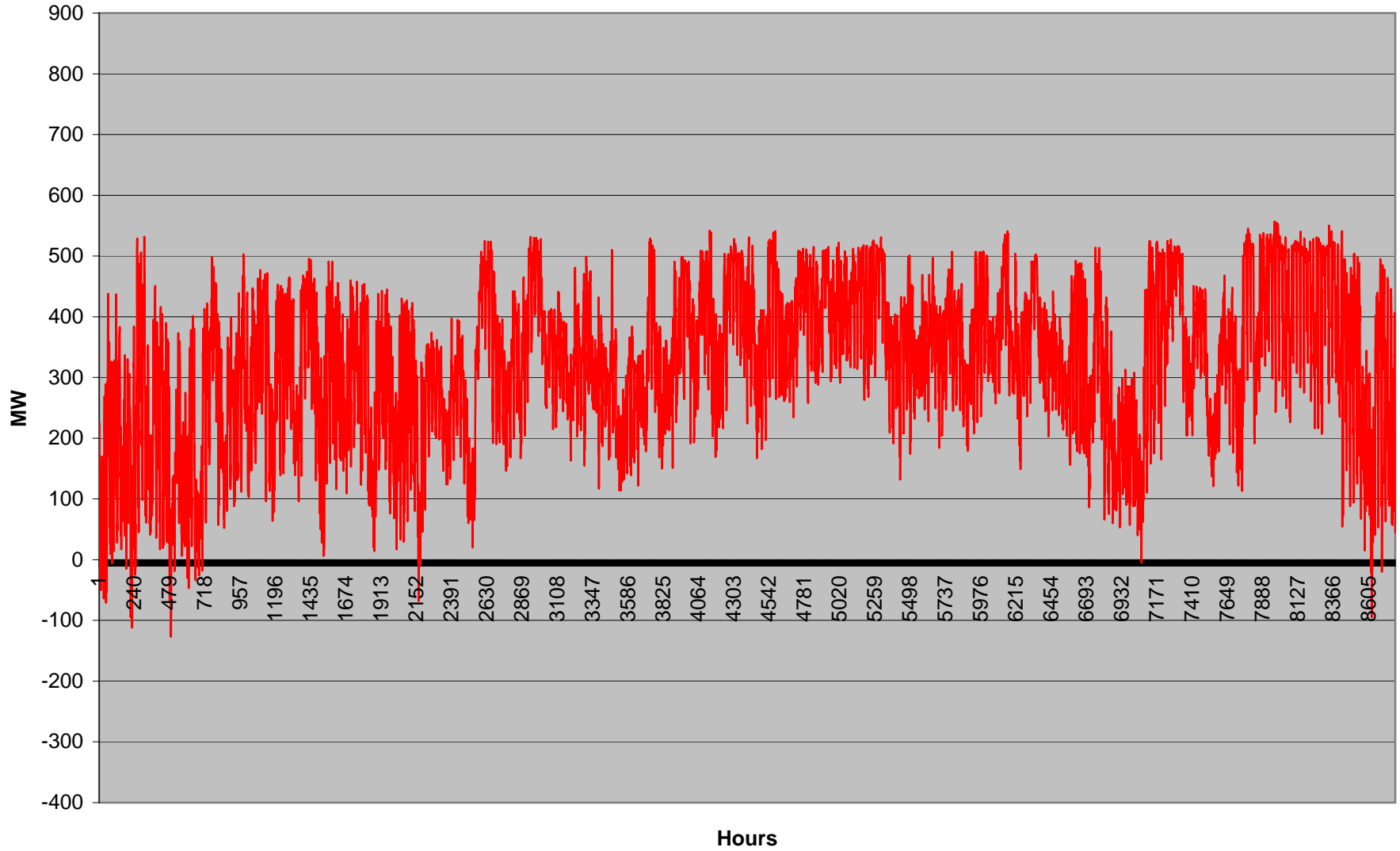
Base Case Alternative: Arrowhead-Weston 345kV Line Flow
