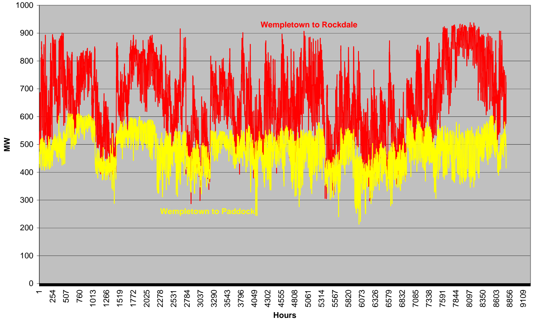
Base Case Plus Fixes Alternative: Wempletown-Rockdale & Wempl.-Paddock 345 kV Flows
