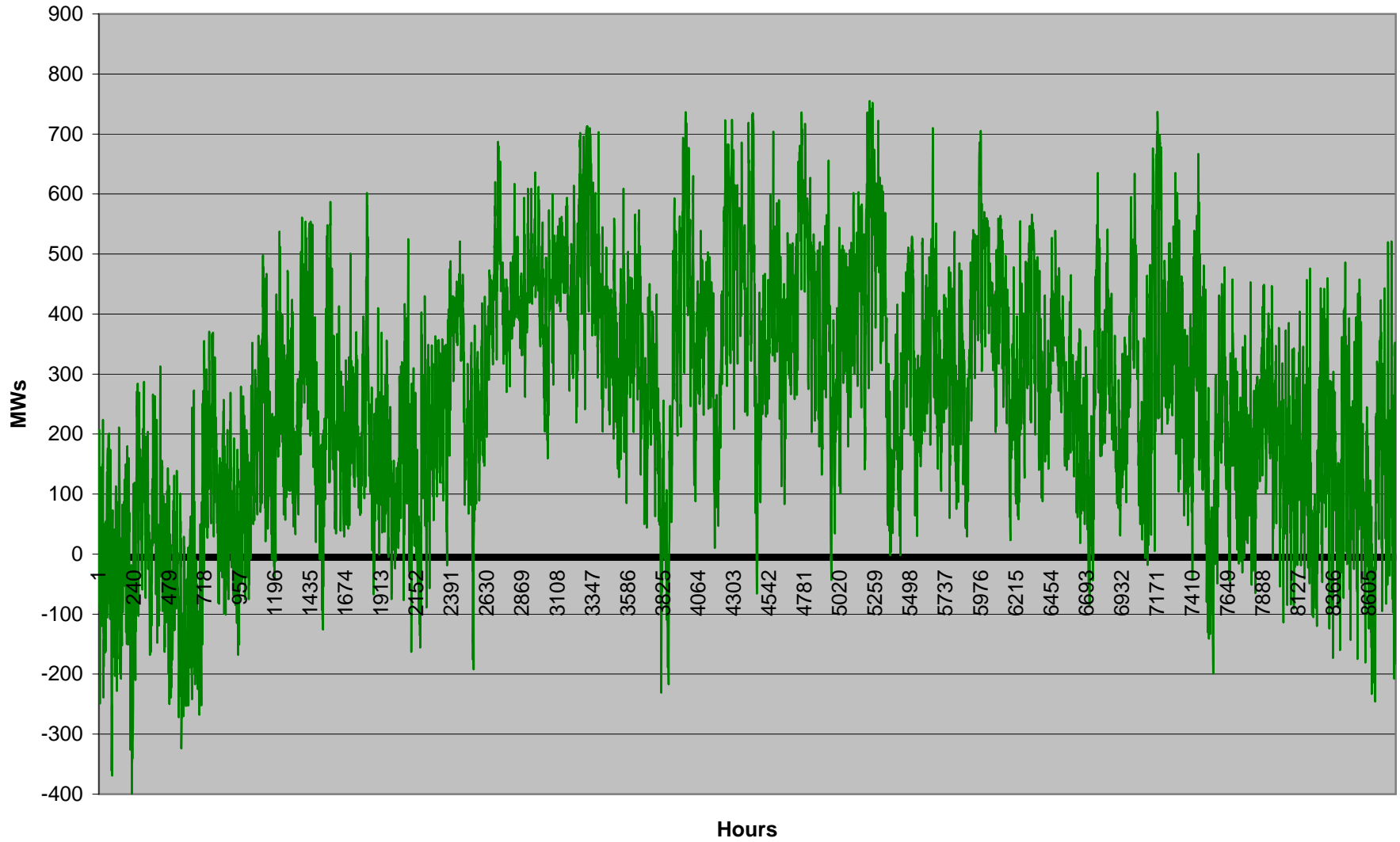
Base Case Plus Fixes Alternative: Eau Claire-Arpin 345 kV Line Flow
