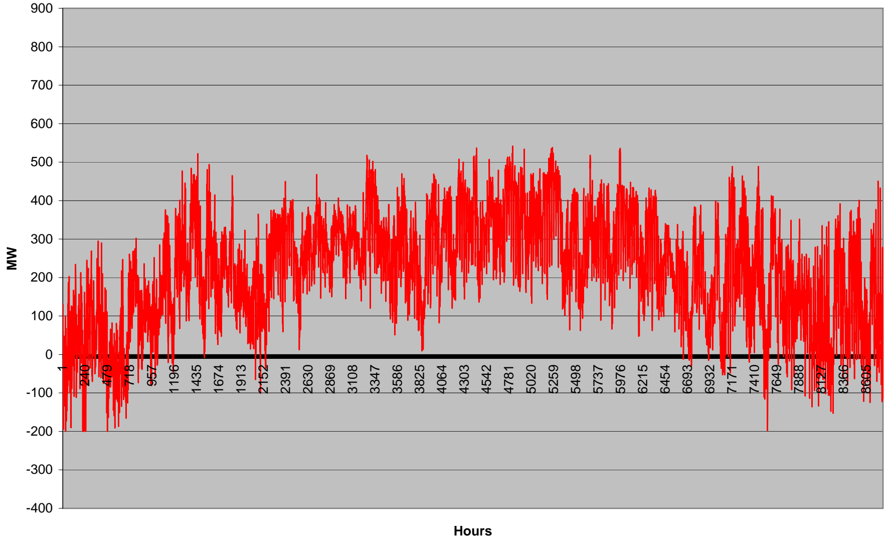
Base Case Plus Fixes Alternative: Arrowhead-Weston 345kV Line Flow
