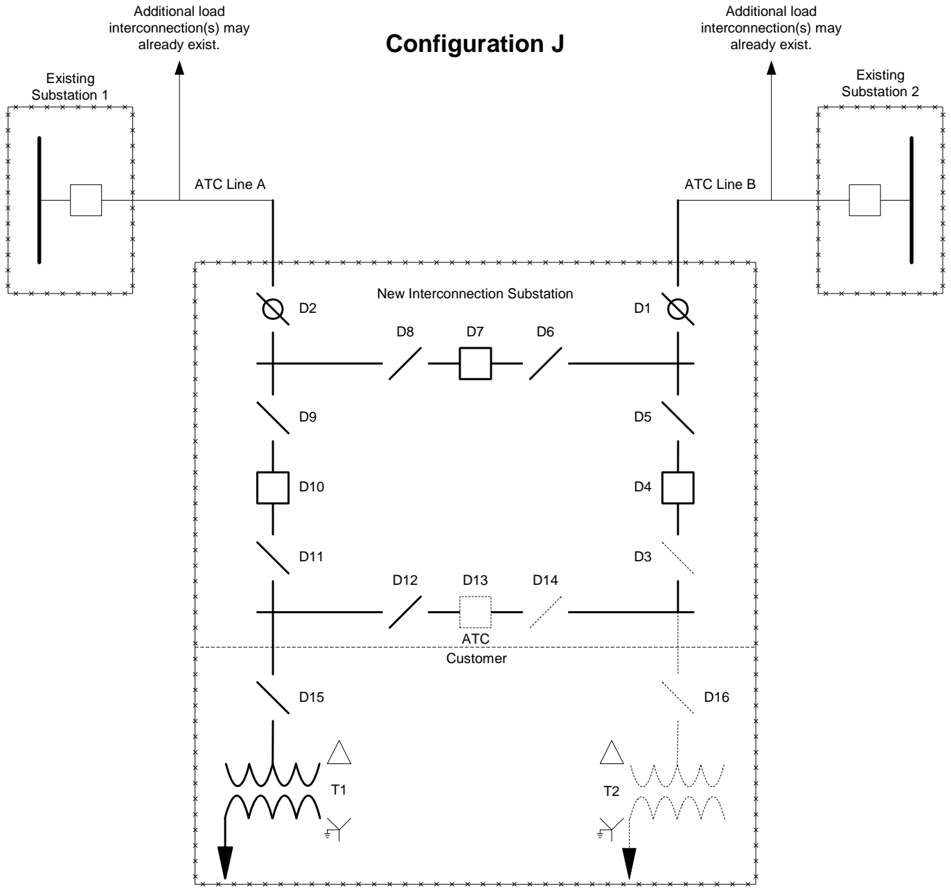
Figure F.10: Load Interconnection Configuration J
