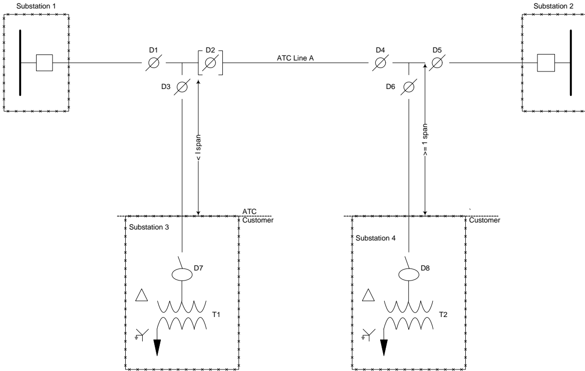
Figure 1: Typical switch installation on a line with multiple radials taps 21
