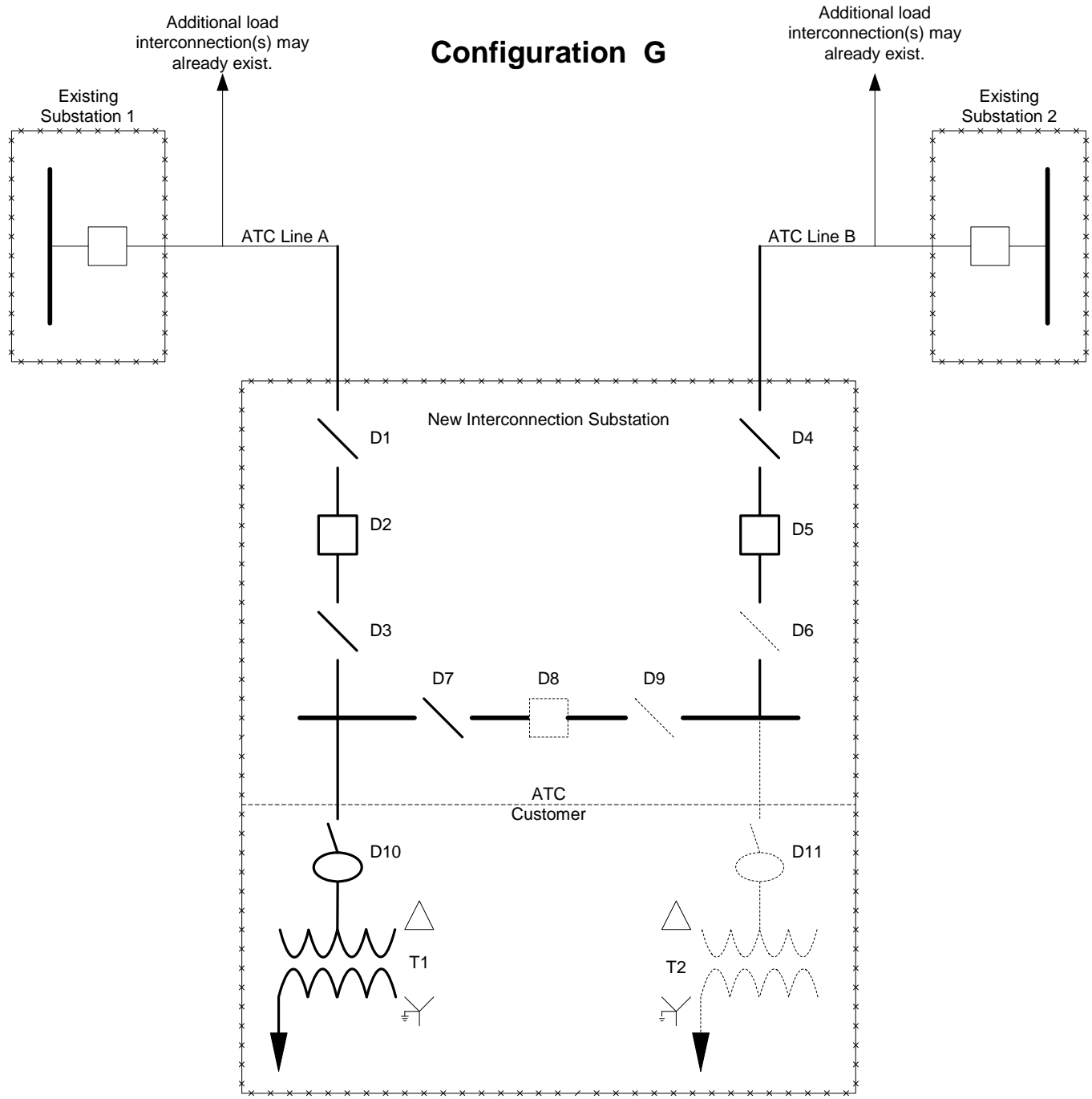
Figure F.8: Load Interconnection Configuration G
