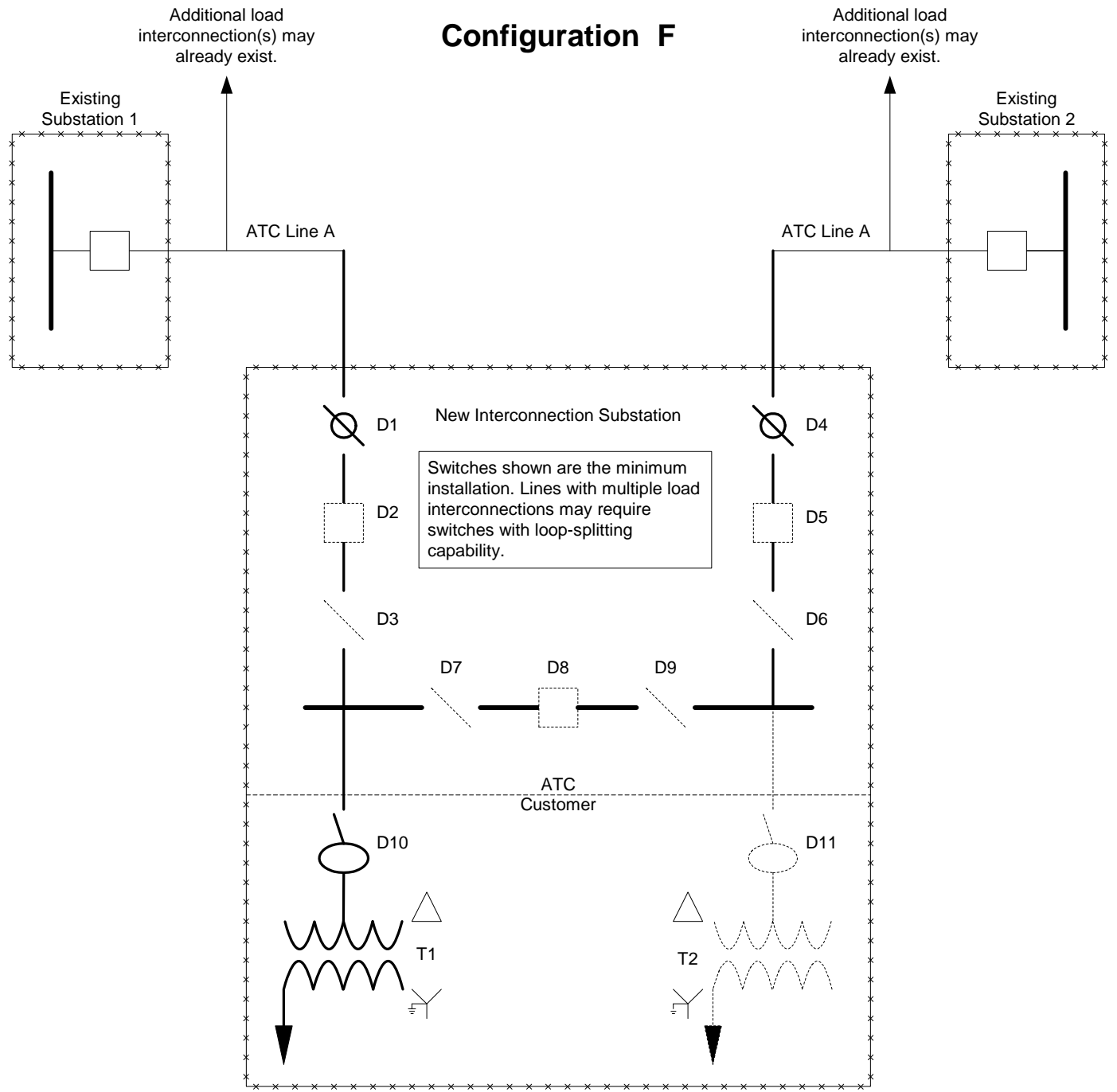
Figure F.7: Load Interconnection Configuration F
