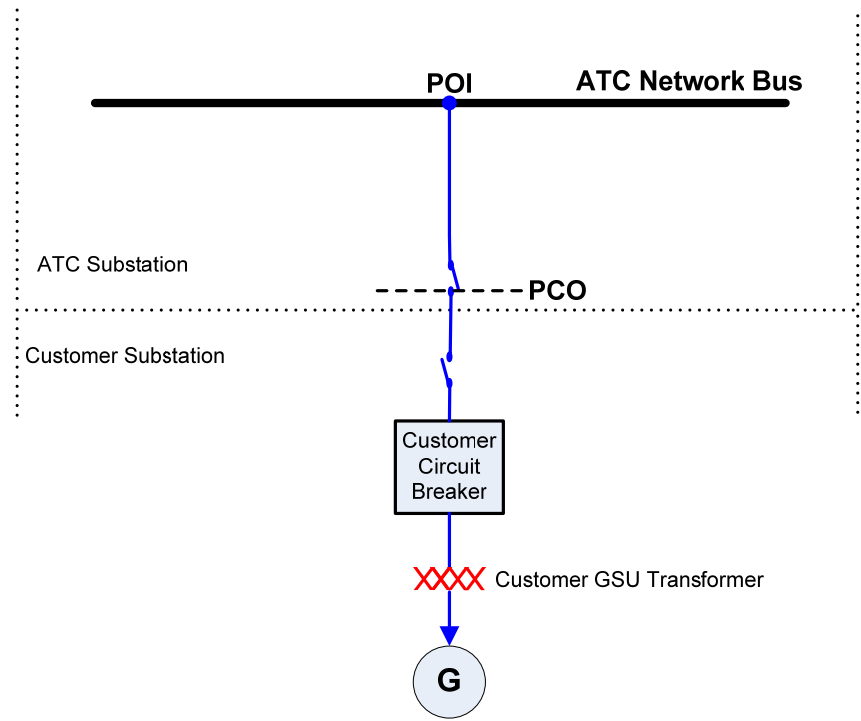
Figure 3-1: Minimum Configuration
