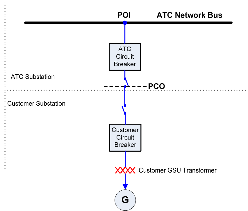
Figure 3-2: Alternate Configuration
